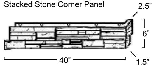
Stacked Stone Corner Panel
