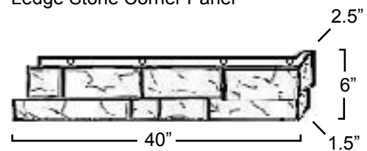
Ledge Stone Corner Panel
